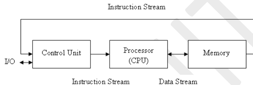
Figure 1.8 SISD
